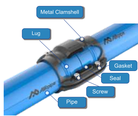
Lugged Ring Clamping Style Connection DN63 - Dn200mm
